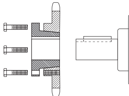
Reverse mounting
