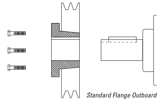
Standard Flange Outboard
