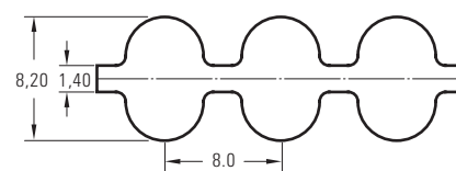
Standard Belt Width
