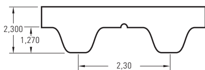
Standard Belt Width
